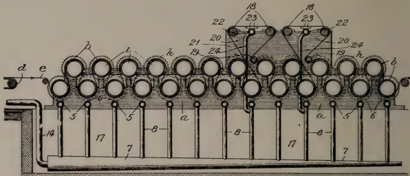
Vertical Section of a novel Paper Drying Apparatus recently patented by the H. W. Johns-Manville Co. View shows the paper passing over or through the rolls, another means of applying air directly to the paper.
